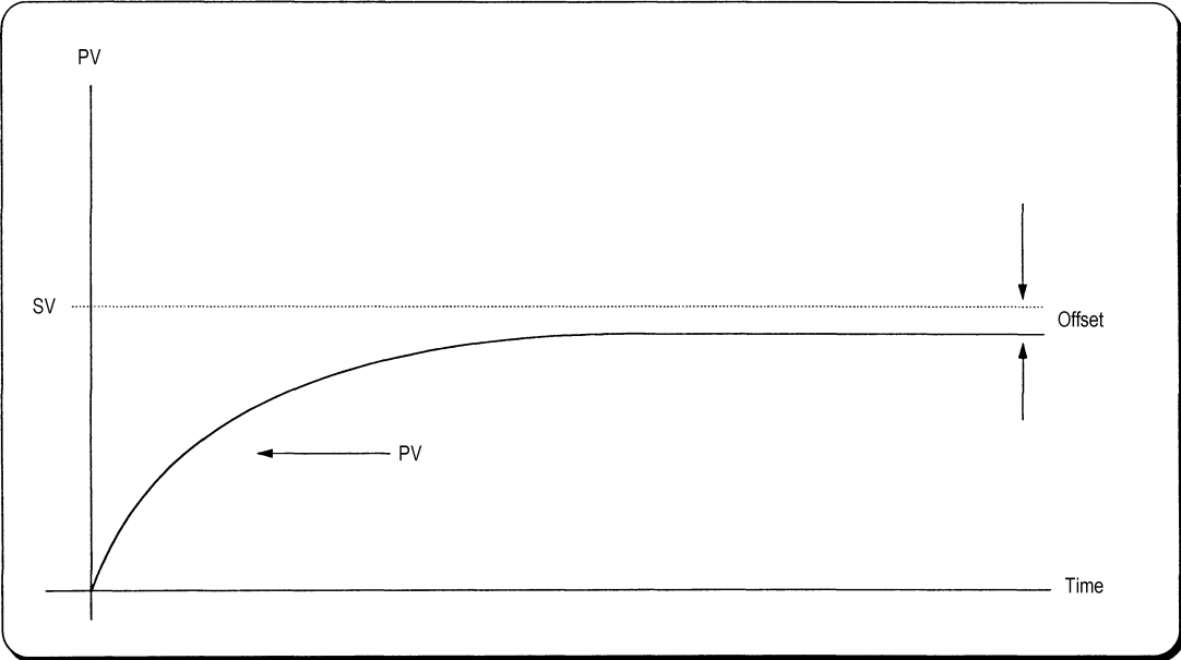
Fig. 2.1 When the proportional constant ( K_p ) is small
