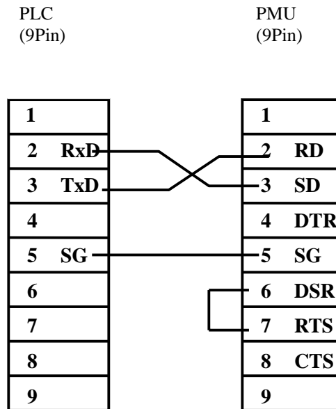
B-3-1-2-4. Cable connection (PMU↔ PLC)
